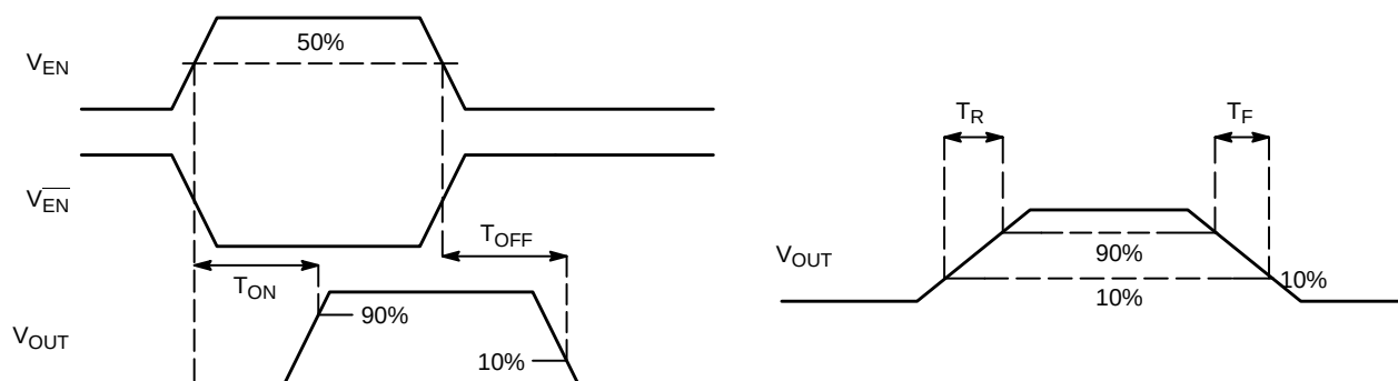
Figure 4. Voltage Waveform
