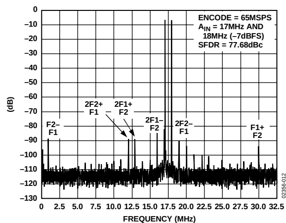
Figure 17. Two Tone @ 17 MHz and 18 MHz
