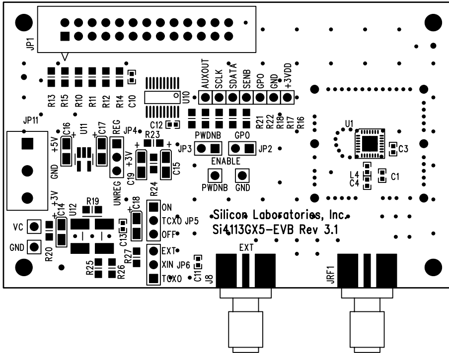
Figure 31. Si4113GX5-BM Silkscreen
