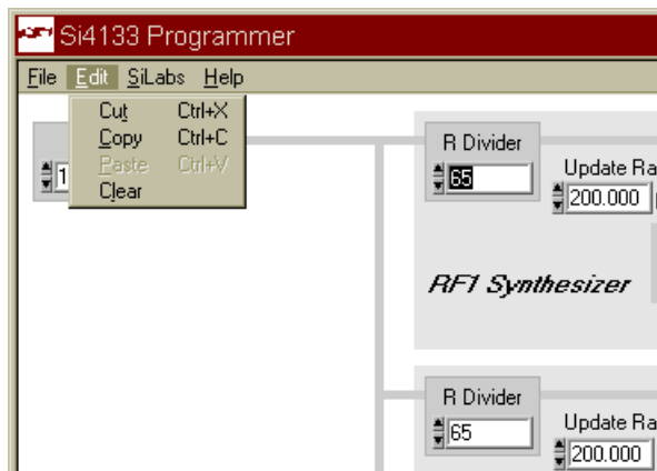
Figure 4. Edit Menu
