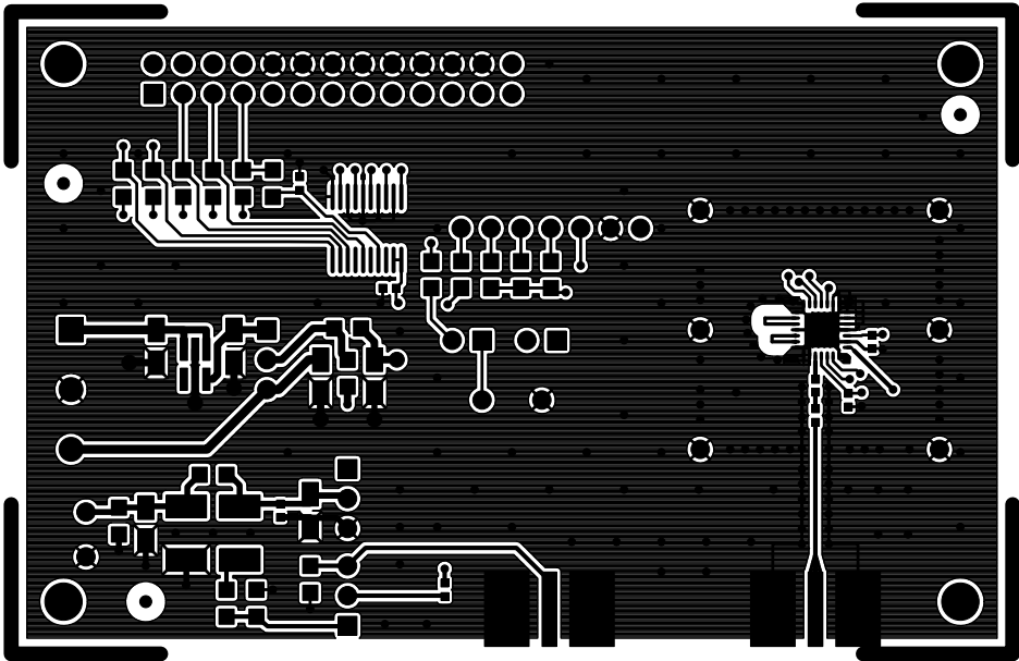
Figure 32. Si4113GX5-BM Component
