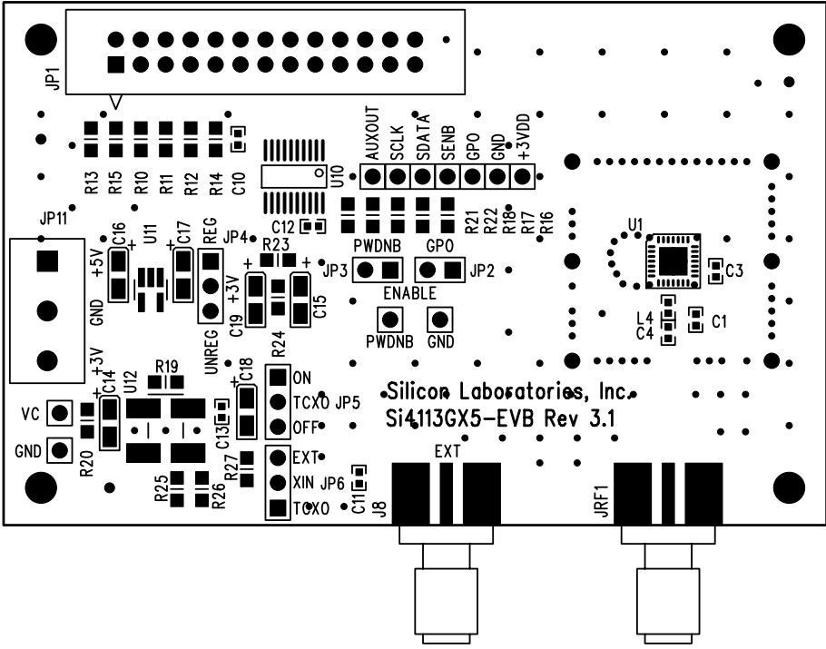
Figure 31. Si4113GX5-BM Silkscreen
