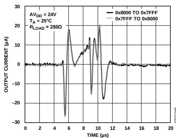
Figure 35. Digital-to-Analog Glitch
