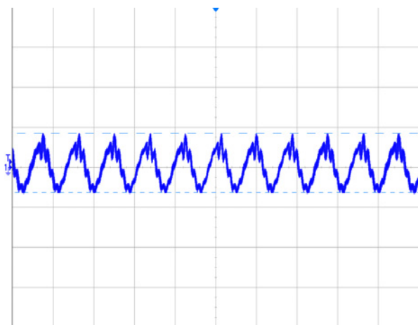
Figure 4 Output ripple & noise (5 \mu s/div, 100mV/div), see Figure 18 for test configuration
