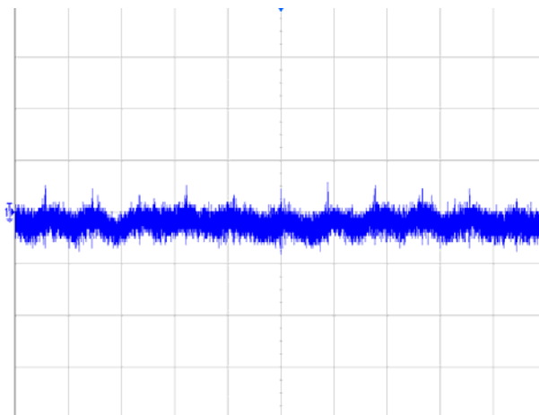
Figure 5 Input reflected ripple current (5 \mu s/div, 20mA/div), see Figure 18 for test configuration
