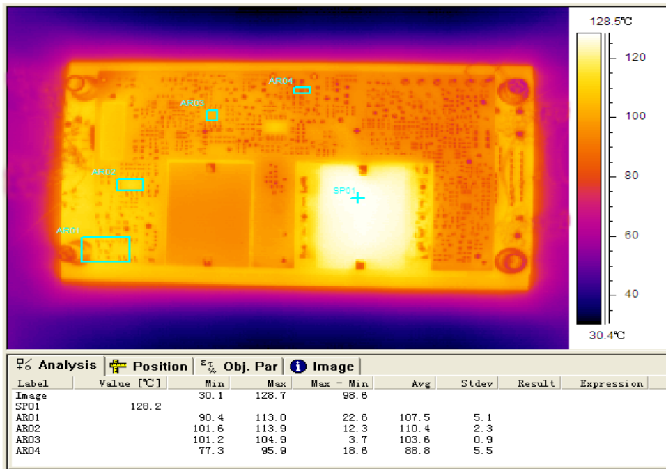
Figure 3 Thermal image, 24\text{V}_{in} , 28\text{V}_o , full load, room temperature
