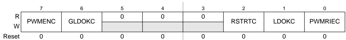
Figure 14-34. PMF Enable Control C Register (PMFENCC)
