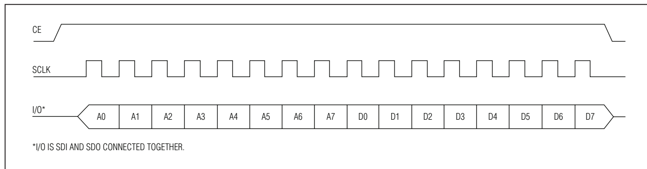
Figure 11. 3-Wire Single-Byte Transfer
