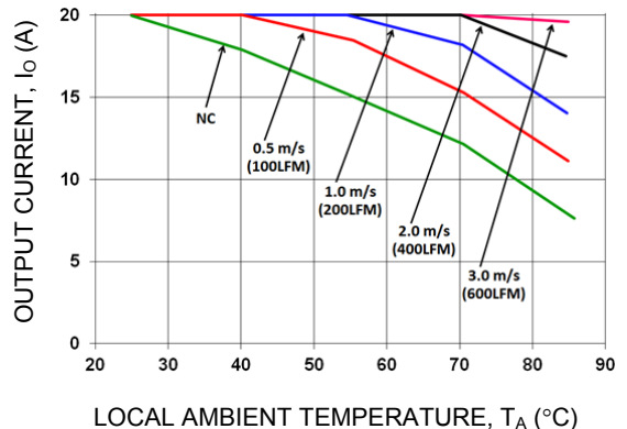
Figure 22. Output Current Derating for the Base Plate EBDW020A0Bxx-H and 0.25 inch heat sink in the Transverse Orientation; Airflow Direction from Vin(-) to Vin(+); Vin = 48V.
