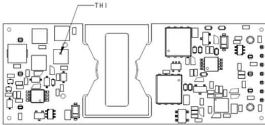
Figure 18. Location of the thermal reference temperature TH. Do not exceed 113 °C.
