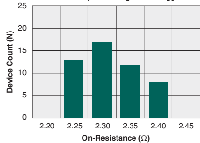
Typical On-Resistance Distribution (N=50, I_F=5mA , I_L=350mA_{DC} )
