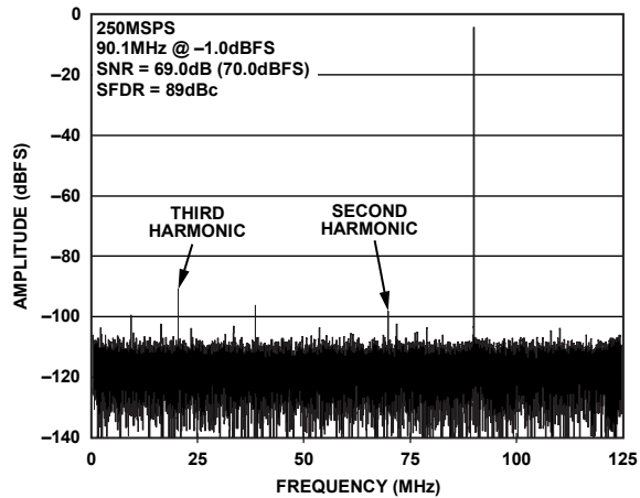
Figure 28. AD9634-250 Single-Tone FFT with f_{IN} = 90.1 MHz
