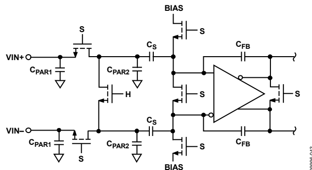
Figure 46. Switched-Capacitor Input
