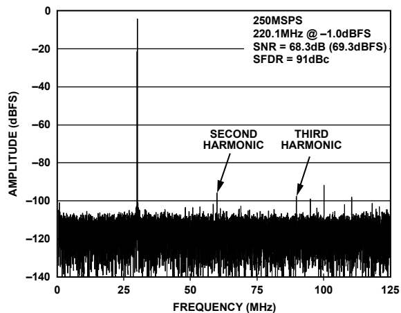
Figure 30. AD9634-250 Single-Tone FFT with f_{IN} = 220.1 MHz
