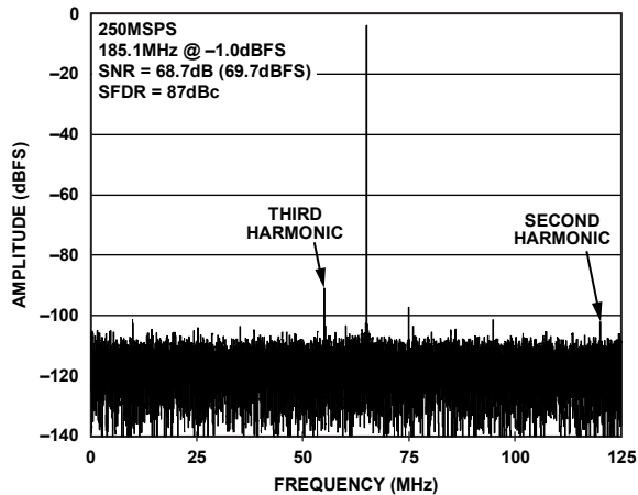
Figure 29. AD9634-250 Single-Tone FFT with f_{IN} = 185.1 MHz
