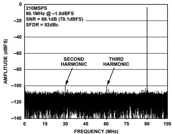
Figure 16. AD9634-210 Single-Tone FFT with f_{IN} = 90.1 MHz
