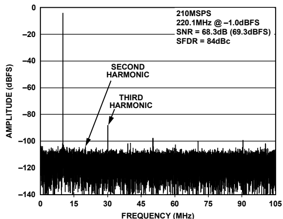
Figure 18. AD9634-210 Single-Tone FFT with f_{IN} = 220.1 MHz
