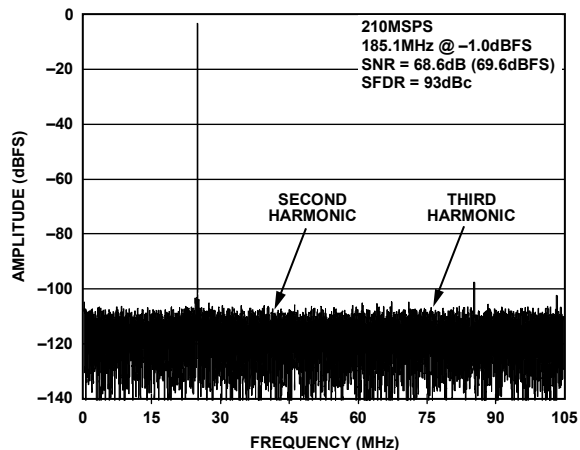
Figure 17. AD9634-210 Single-Tone FFT with f_{IN} = 185.1 MHz
