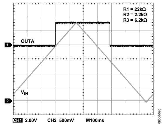
Figure 27. Hysteresis Programmed to ~513 mV at Top of Input String (Hysteresis at ADCMP341 Pins \approx 104 mV)
