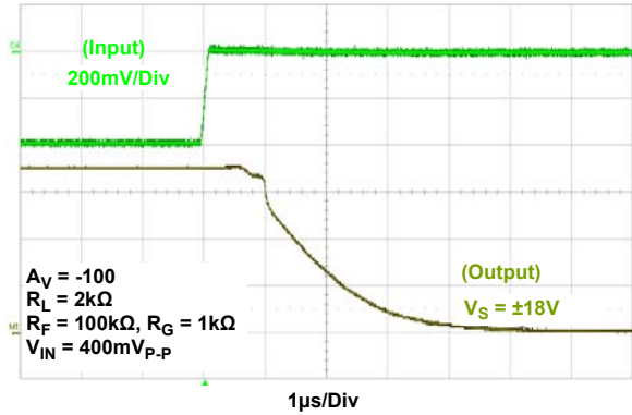
Figure 45. Saturation Recovery ( V_S = \pm 18V )
