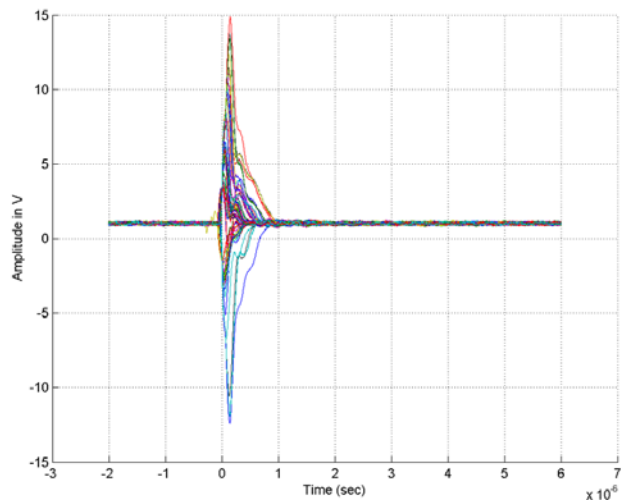
Figure 61. SET Response with V_S = \pm 15.0\text{V}
