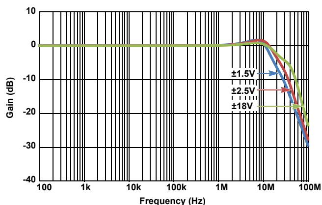
Figure 40. Frequency Response vs Supply Voltage
