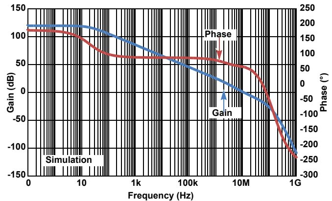
Figure 30. Open-Loop Frequency Response ( C_L = 10pF )
