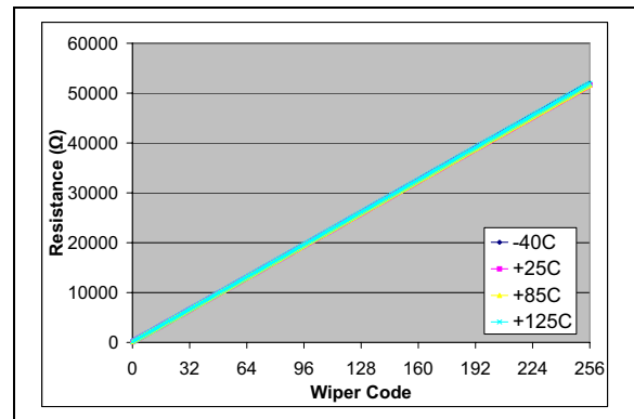
FIGURE 2-43: 50 kΩ – R_{WB} ( \Omega ) vs. Wiper Setting and Ambient Temperature ( V_{DD} = 3.0\text{V} , I_W = 48\text{ }\mu\text{A} ).
