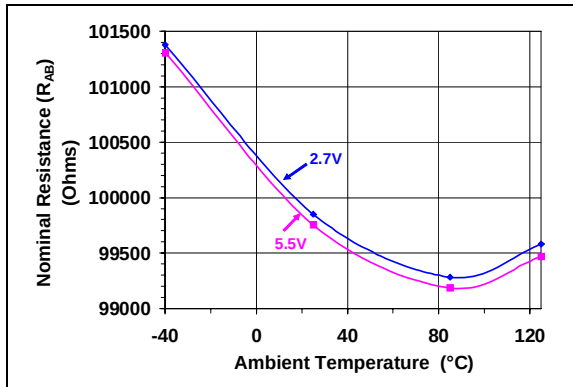
FIGURE 2-56: 100 k \Omega – Nominal Resistance ( R_{AB} ) ( \Omega ) vs. Ambient Temperature and V_{DD} .
