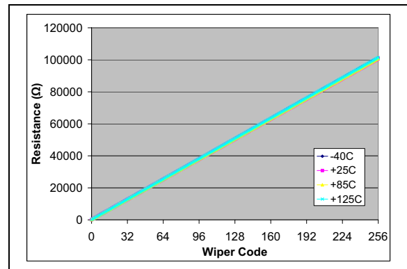
FIGURE 2-58: 100 k \Omega – R_{WB} ( \Omega ) vs. Wiper Setting and Ambient Temperature ( V_{DD} = 3.0\text{V} , I_W = 24\text{ }\mu\text{A} ).
