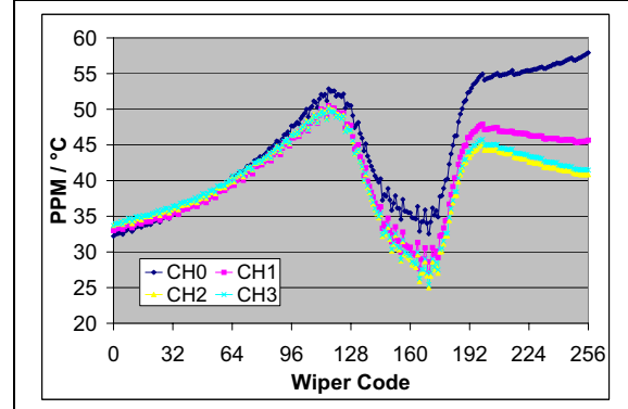
FIGURE 2-32: 10 kΩ – R_{WB} PPM/°C vs. Wiper Setting. ( R_{BW(\text{code}=n, 125^\circ\text{C})} - R_{BW(\text{code}=n, -40^\circ\text{C})} / R_{BW(\text{code}=256, 25^\circ\text{C})} / 165^\circ\text{C} * 1,000,000 ) ( V_{DD} = 3.0\text{V} , I_W = 150\text{ }\mu\text{A} ).
