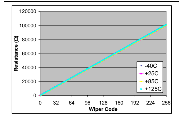
FIGURE 2-57: 100 k \Omega – R_{WB} ( \Omega ) vs. Wiper Setting and Ambient Temperature ( V_{DD} = 5.5\text{V} , I_W = 45\text{ }\mu\text{A} ).
