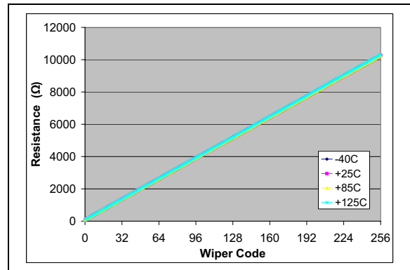
FIGURE 2-27: 10 kΩ – R_{WB} (Ω) vs. Wiper Setting and Ambient Temperature ( V_{DD} = 5.5\text{V} , I_W = 150\text{ μA} ).
