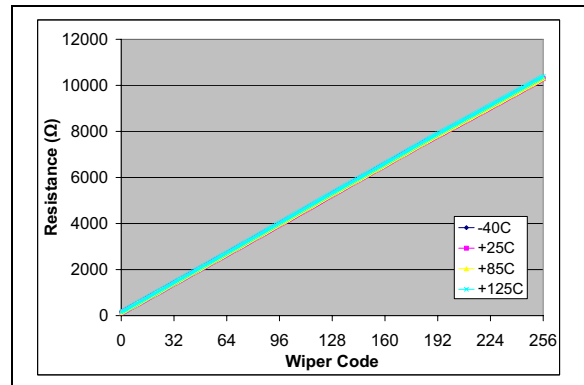
FIGURE 2-28: 10 kΩ – R_{WB} (Ω) vs. Wiper Setting and Ambient Temperature ( V_{DD} = 3.0\text{V} , I_W = 150\text{ μA} ).
