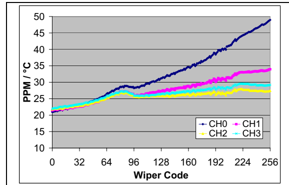
FIGURE 2-31: 10 kΩ – R_{WB} PPM/°C vs. Wiper Setting. ( R_{BW(\text{code}=n, 125^\circ\text{C})} - R_{BW(\text{code}=n, -40^\circ\text{C})} / R_{BW(\text{code}=256, 25^\circ\text{C})} / 165^\circ\text{C} * 1,000,000 ) ( V_{DD} = 5.5\text{V} , I_W = 150\text{ }\mu\text{A} ).
