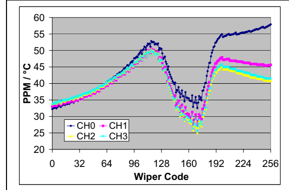
FIGURE 2-32: 10 kΩ – R_{WB} PPM/°C vs. Wiper Setting. ( R_{BW(\text{code}=n, 125^\circ\text{C})} - R_{BW(\text{code}=n, -40^\circ\text{C})} / R_{BW(\text{code}=256, 25^\circ\text{C})} / 165^\circ\text{C} * 1,000,000 ) ( V_{DD} = 3.0\text{V} , I_W = 150\text{ }\mu\text{A} ).
