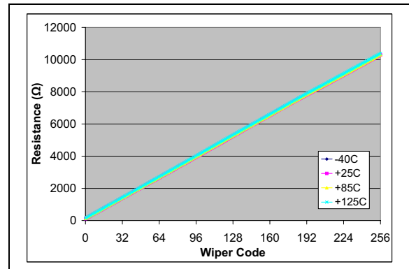
FIGURE 2-28: 10 k \Omega – R_{WB} ( \Omega ) vs. Wiper Setting and Ambient Temperature ( V_{DD} = 3.0\text{V} , I_W = 150\text{ }\mu\text{A} ).
