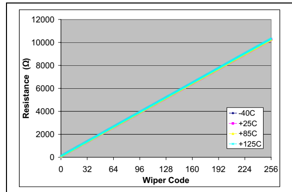
FIGURE 2-27: 10 k \Omega – R_{WB} ( \Omega ) vs. Wiper Setting and Ambient Temperature ( V_{DD} = 5.5\text{V} , I_W = 150\text{ }\mu\text{A} ).
