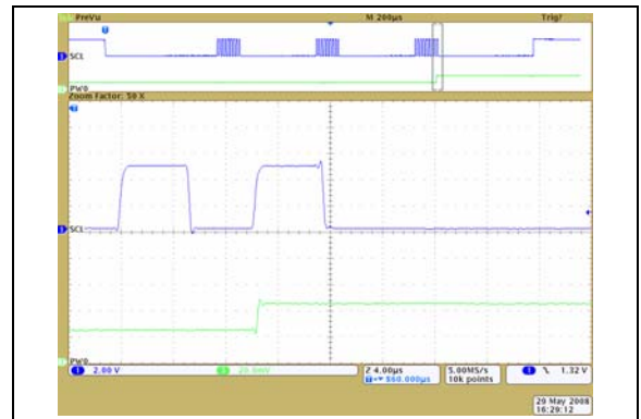
FIGURE 2-36: 10\text{ k}\Omega – Low-Voltage Increment Wiper Settling Time ( V_{DD} = 5.5\text{V} ) ( 1\text{ }\mu\text{s/Div} ).
