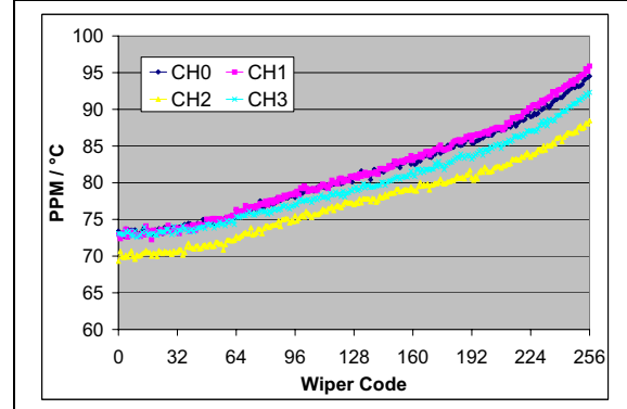
FIGURE 2-16: 5\text{ k}\Omega – R_{WB} PPM/ ^\circ\text{C} vs. Wiper Setting. ( R_{BW(\text{code}=n, 125^\circ\text{C})} - R_{BW(\text{code}=n, -40^\circ\text{C})} / R_{BW(\text{code}=256, 25^\circ\text{C})} / 165^\circ\text{C} * 1,000,000 ) ( V_{DD} = 3.0\text{V} , I_W = 190\text{ }\mu\text{A} ).
