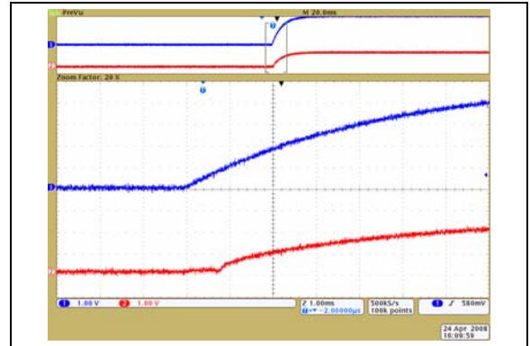
FIGURE 2-35: 10\text{ k}\Omega – Low-Voltage Increment Wiper Settling Time ( V_{DD} = 2.7\text{V} ) ( 1\text{ }\mu\text{s/Div} ).
