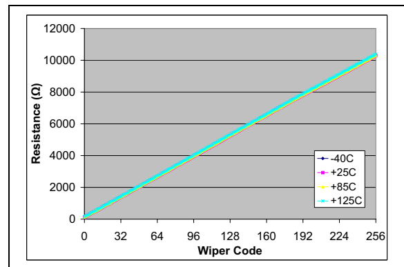
FIGURE 2-28: 10 kΩ – R_{WB} ( \Omega ) vs. Wiper Setting and Ambient Temperature ( V_{DD} = 3.0\text{V} , I_W = 150\text{ }\mu\text{A} ).
