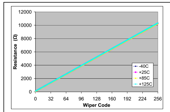
FIGURE 2-27: 10 kΩ – R_{WB} ( \Omega ) vs. Wiper Setting and Ambient Temperature ( V_{DD} = 5.5\text{V} , I_W = 150\text{ }\mu\text{A} ).
