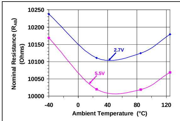
FIGURE 2-26: 10 kΩ – Nominal Resistance ( R_{AB} ) ( \Omega ) vs. Ambient Temperature and V_{DD} .
