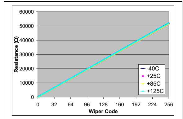
FIGURE 2-43: 50\text{ k}\Omega — R_{WB} ( \Omega ) vs. Wiper Setting and Ambient Temperature ( V_{DD} = 3.0\text{V} , I_W = 48\text{ }\mu\text{A} ).
