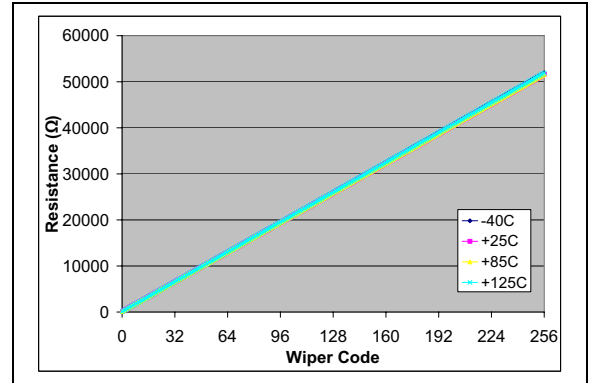
FIGURE 2-42: 50\text{ k}\Omega — R_{WB} ( \Omega ) vs. Wiper Setting and Ambient Temperature ( V_{DD} = 5.5\text{V} , I_W = 90\text{ }\mu\text{A} ).
