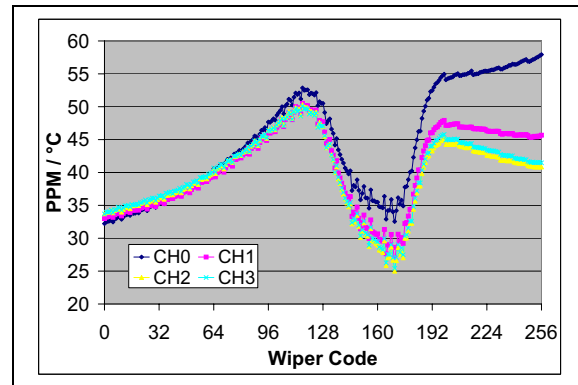
FIGURE 2-32: 10 k \Omega – R_{WB} PPM/ ^\circ\text{C} vs. Wiper Setting. ( R_{BW(\text{code}=n, 125^\circ\text{C})} - R_{BW(\text{code}=n, -40^\circ\text{C})} / R_{BW(\text{code}=256, 25^\circ\text{C})} / 165^\circ\text{C} * 1,000,000 ) ( V_{DD} = 3.0\text{V} , I_W = 150\text{ }\mu\text{A} ).
