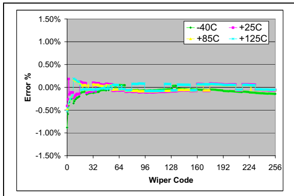
FIGURE 2-30: 10 k \Omega – Worst Case R_{BW} from Average R_{BW} ( R_{BW0} - R_{BW3} ) Error (%) vs. Wiper Setting and Temperature ( V_{DD} = 3.0\text{V} , I_W = 150\text{ }\mu\text{A} ).
