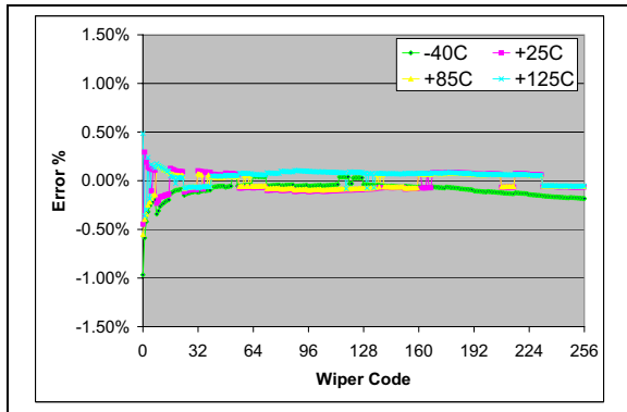
FIGURE 2-29: 10 k \Omega – Worst Case R_{BW} from Average R_{BW} ( R_{BW0} - R_{BW3} ) Error (%) vs. Wiper Setting and Temperature ( V_{DD} = 5.5\text{V} , I_W = 150\text{ }\mu\text{A} ).
