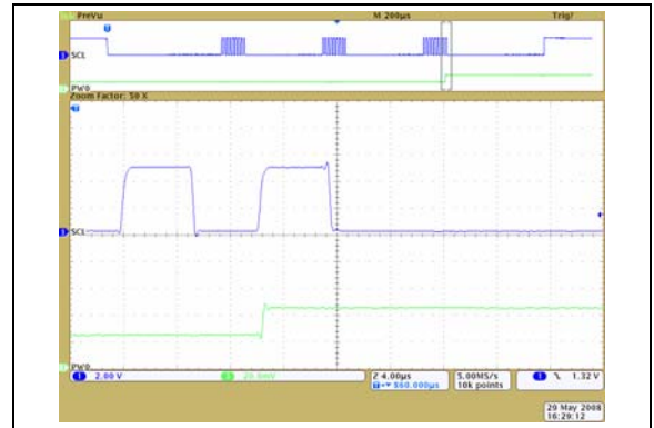
FIGURE 2-36: 10 k \Omega – Low-Voltage Increment Wiper Settling Time ( V_{DD} = 5.5\text{V} ) (1 \mu\text{s}/\text{Div} ).
