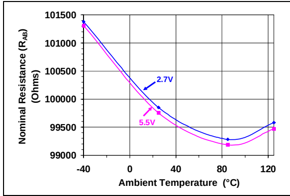
FIGURE 2-56: 100 kΩ – Nominal Resistance ( R_{AB} ) ( \Omega ) vs. Ambient Temperature and V_{DD} .
