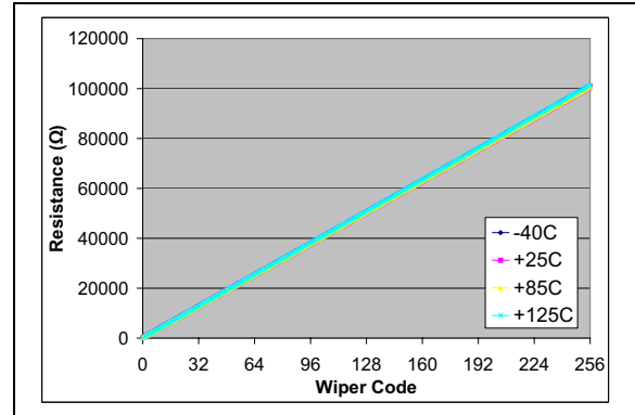
FIGURE 2-57: 100 kΩ – R_{WB} ( \Omega ) vs. Wiper Setting and Ambient Temperature ( V_{DD} = 5.5\text{V} , I_W = 45 \mu\text{A} ).
