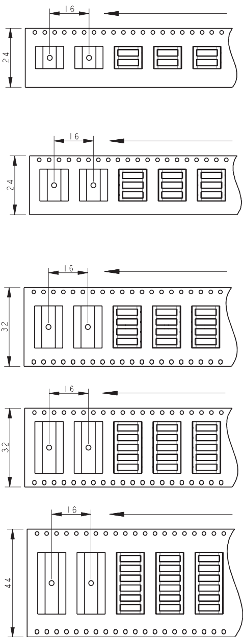
PACKING DETAILS FIXED CONNECTOR
