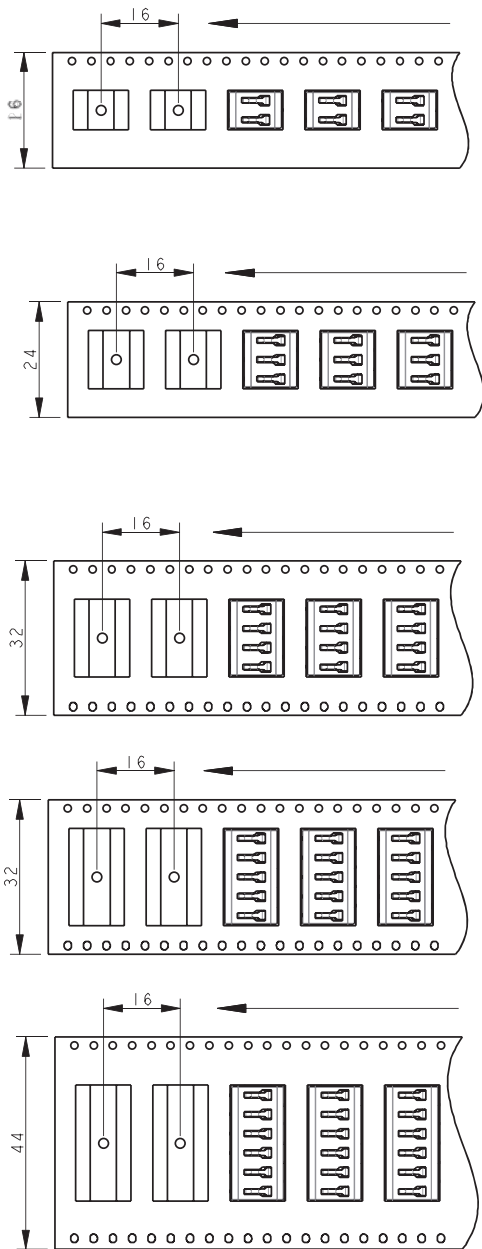
PACKING DETAILS SPRUNG CONNECTOR
