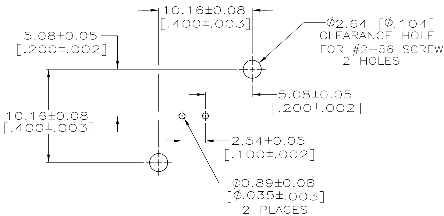
PCB CONFIGURATION
