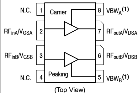
Figure 1. Pin Connections
