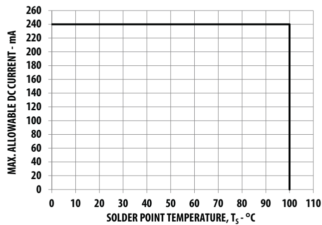
Figure 16 Maximum Forward Current vs. Solder Point Temperature. Derated based on T_{JMAX} = 125^{\circ}\text{C} , R\theta_{J-S} = 15^{\circ}\text{C/W}
