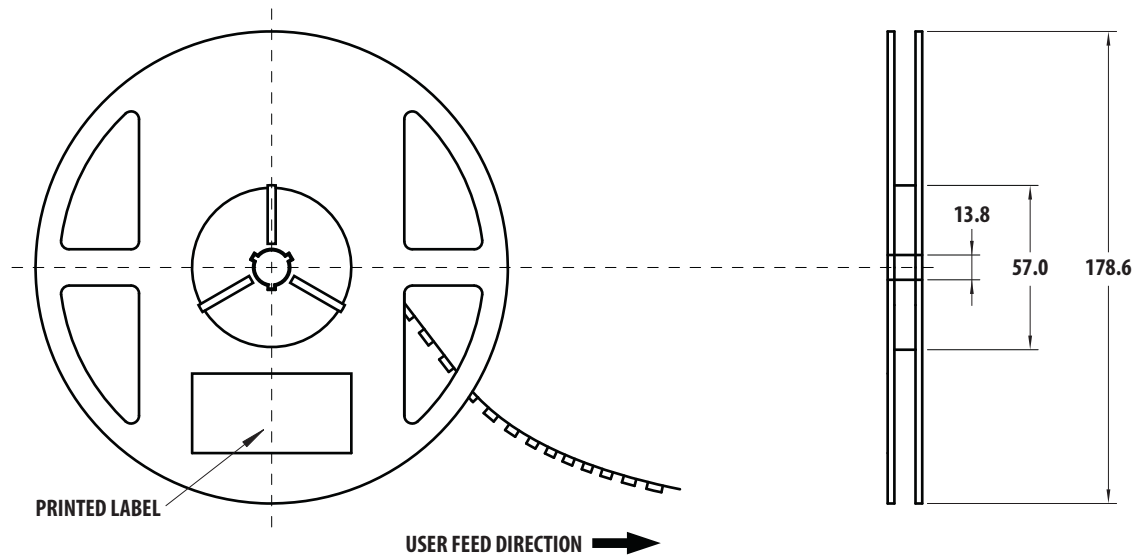
Figure 19 Reel Dimensions
