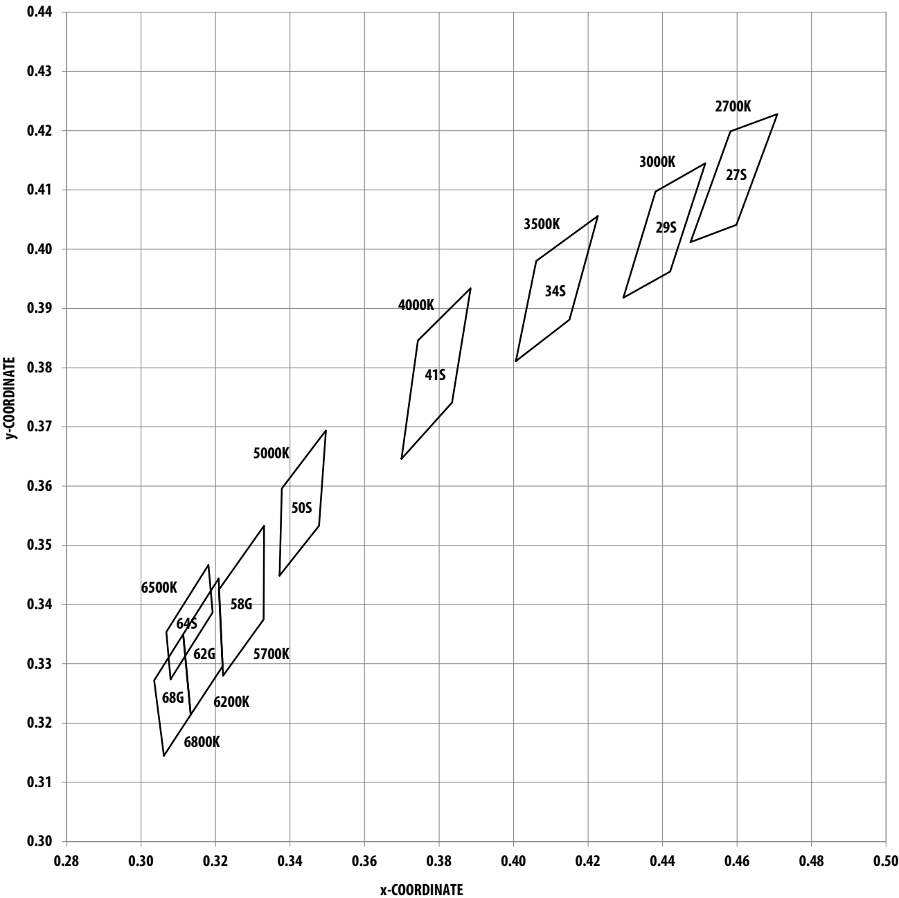
Figure 2 Chromaticity Diagram
