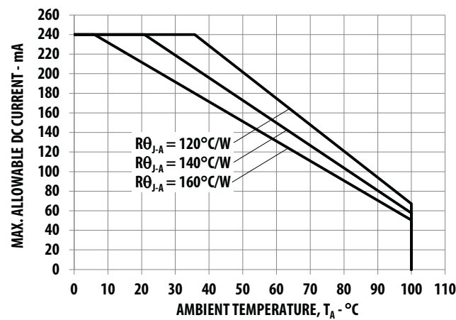
Figure 15 Maximum Forward Current vs. Ambient Temperature. Derated based on T_{JMAX} = 125^{\circ}\text{C} , R\theta_{J-A} = 120^{\circ}\text{C/W} , 140^{\circ}\text{C/W} and 160^{\circ}\text{C/W} .
