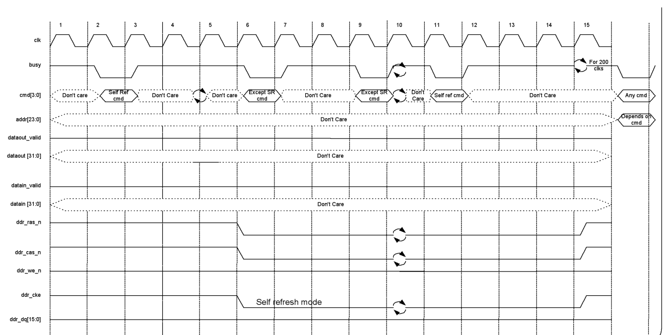
Figure 18. Self Refresh
