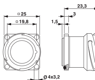
Dimensional drawing
