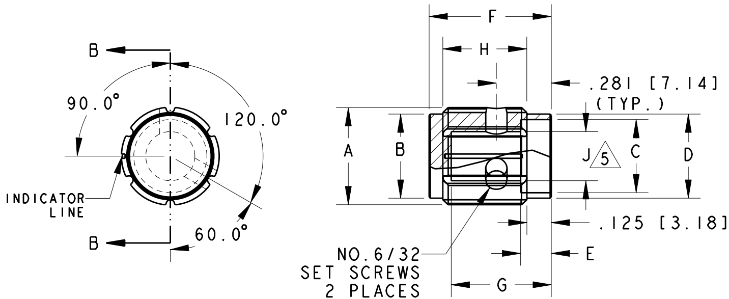
SECTION B-B
