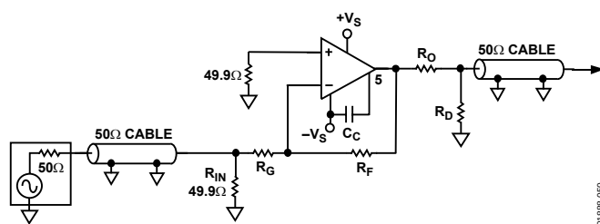
Figure 50. Inverting Gain
