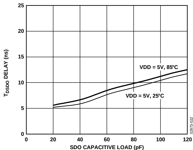
Figure 23. t_{\text{SDO}} Delay vs. Capacitance Load and Supply
