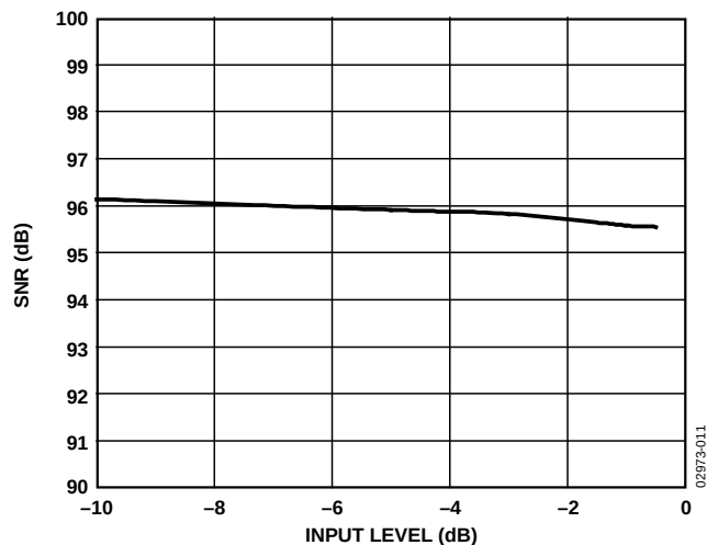
Figure 12. SNR vs. Input Level
