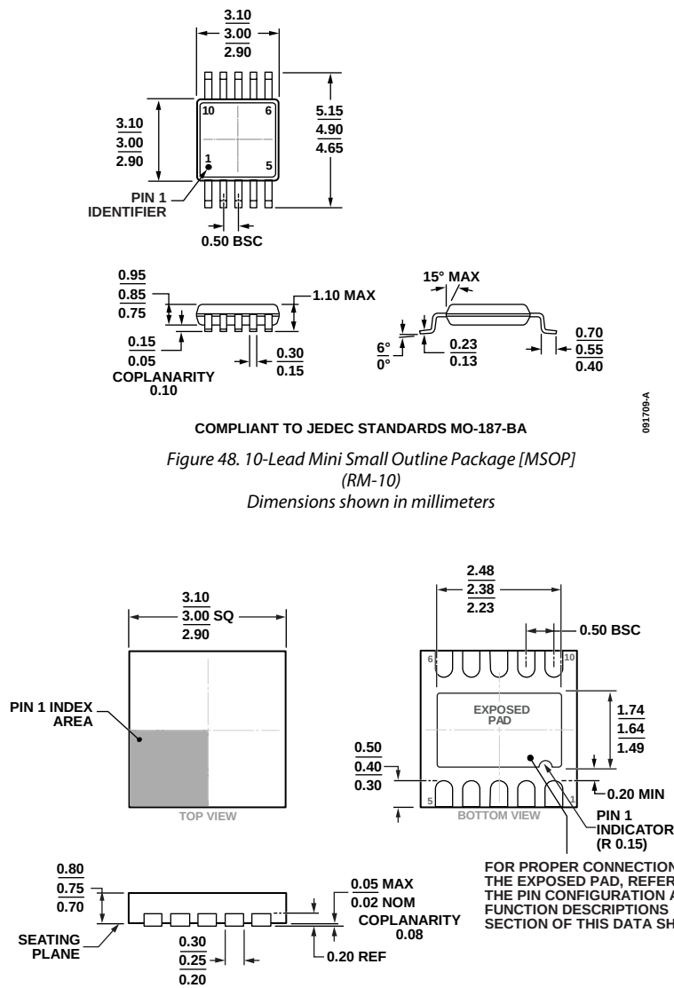
Figure 49. 10-Lead Lead Frame Chip Scale Package [LFCSP_WD] 3 mm x 3 mm Body, Very Very Thin, Dual Lead (CP-10-9) Dimensions shown in millimeters
