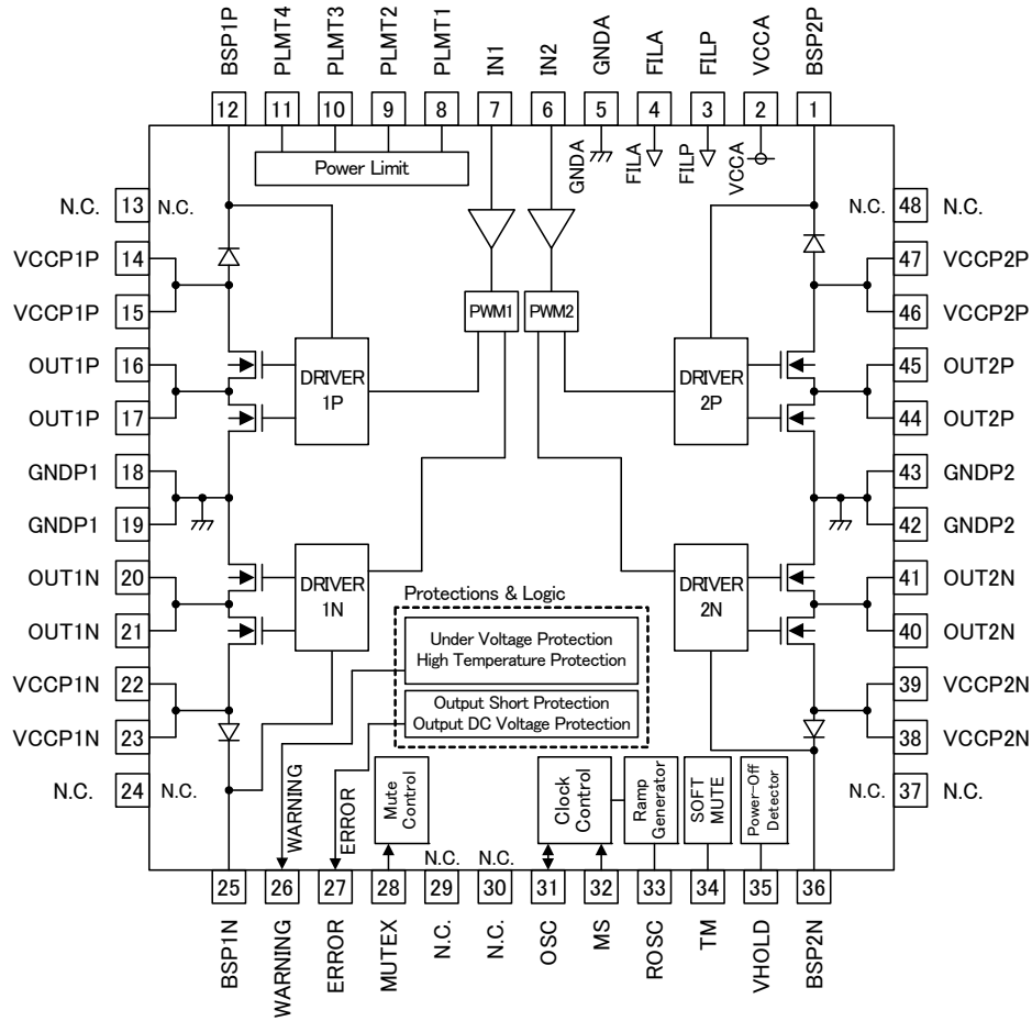
Fig. 23 Pin Assignment Diagram
