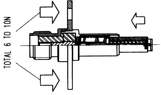
figure 2 (2:1)
