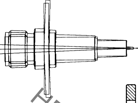
figure 3 (2:1)
