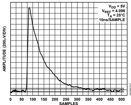
Figure 21. Glitch Energy
