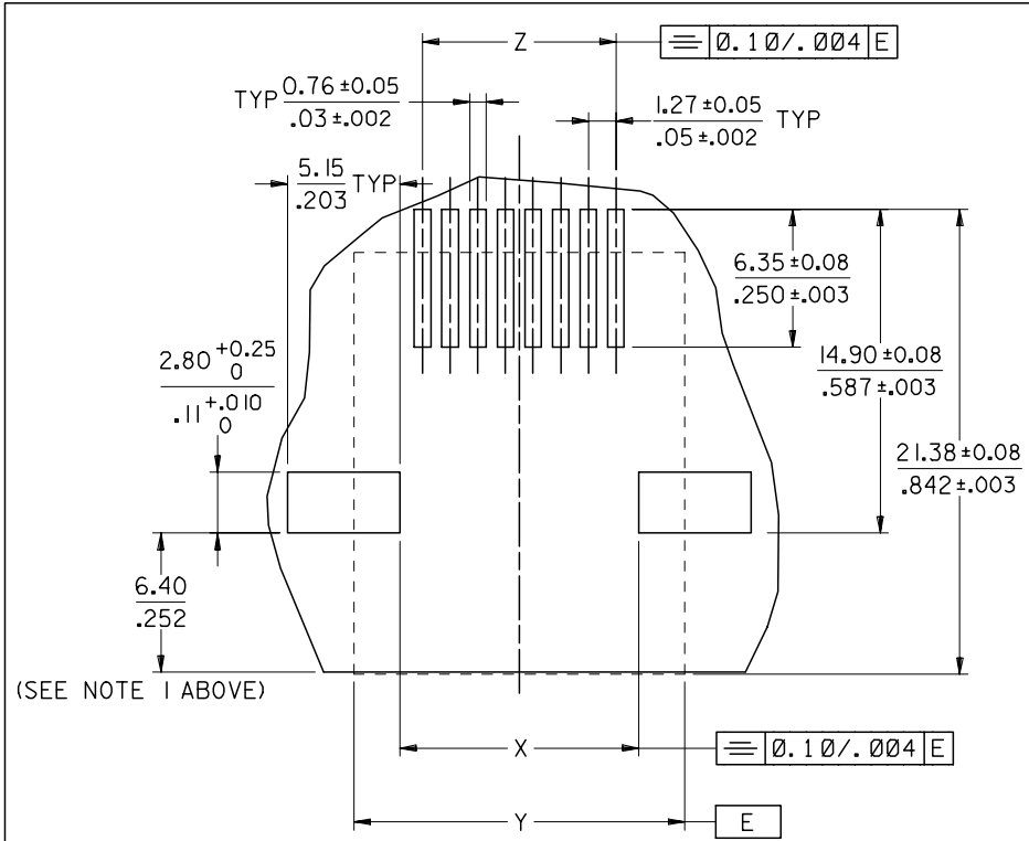
P.C.B. MOUNTING PATTERNS (SOLDER TABS VERSION) VIEW FROM COMPONENT SIDE (SCALE 4:1)
