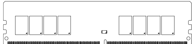
Figure 1: 288-Pin UDIMM (MO-309, R/C-B1)
