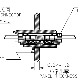
嵌合状態図 MATED & MOUNTED CONNECTOR
