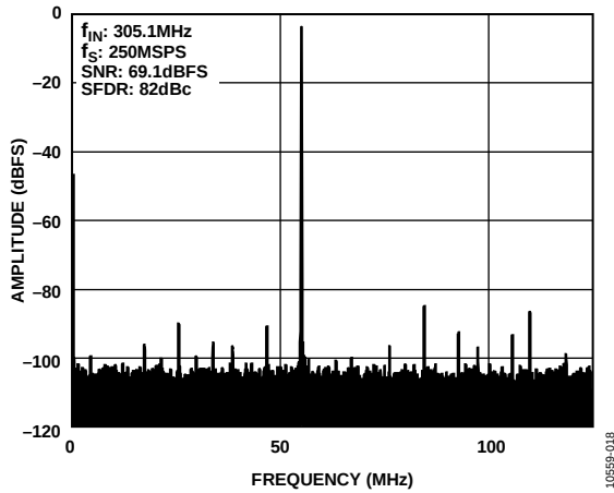
Figure 18. AD9250-250 Single-Tone FFT with f_{IN} = 305.1 MHz
