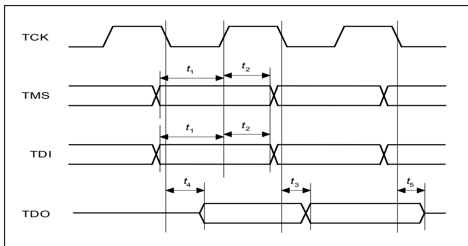
Figure 44 JTAG Timing
