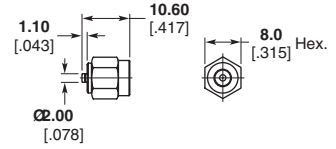
Part No. 1775228-1
