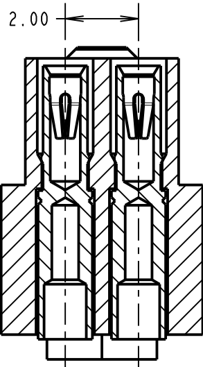
SECTION X-X
