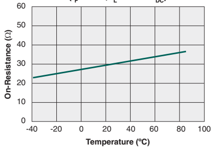
Form-B Typical On-Resistance vs. Temperature ( I_F=5mA, I_L=120mA_{DC} )
