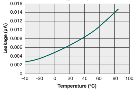
Form-B Typical Leakage vs. Temperature Measured Across Pins 5&6 ( I_F=5mA )
