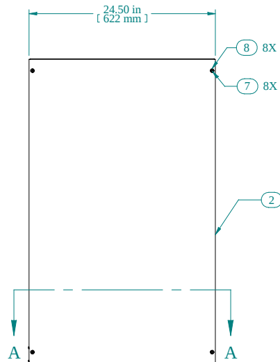
L.S. VIEW
