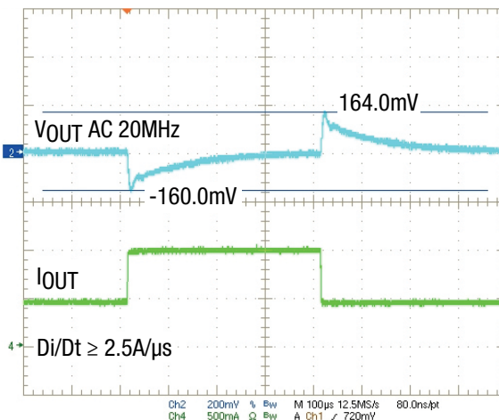
Figure 12. 5\text{V}_{\text{IN}} , 3.3\text{V}_{\text{OUT}} Transient Response, 0.5\text{A} to 1.0\text{A}
