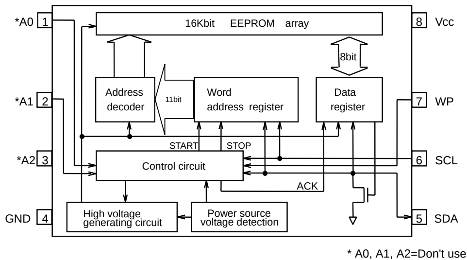
Figure 3. Block diagram
