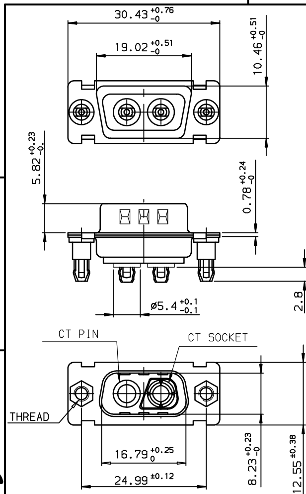
LAYOUT DIMENSIONS (after plating) CONNECTOR SIDE VIEW
