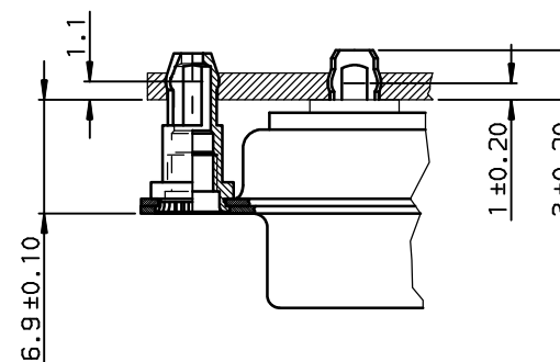
DETAIL OF PRESS FIT Scale: 3
